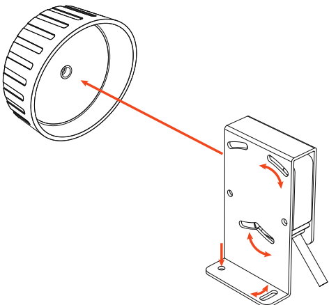
Image 3: Installing and Aligning the Emitter/Receiver and Reflector (horizontal mounted shown)
