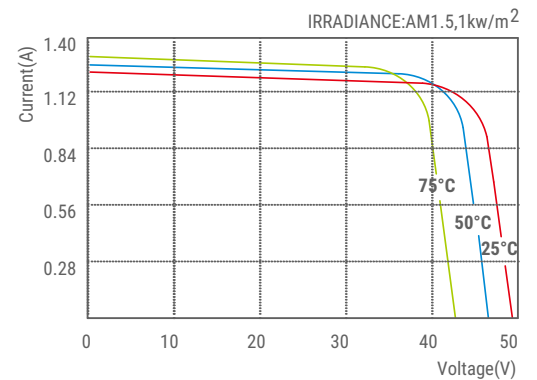
SLP050S-24U I-V Curves
