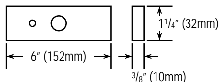
Armature Plate (for E-941SA-300 and E-941SA-300RQ)
