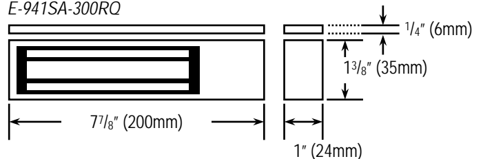
Armature Plate (for E-941SA-300 and E-941SA-300RQ)
