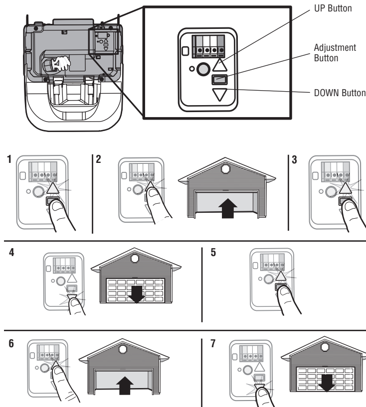
PROGRAMMING BUTTONS
